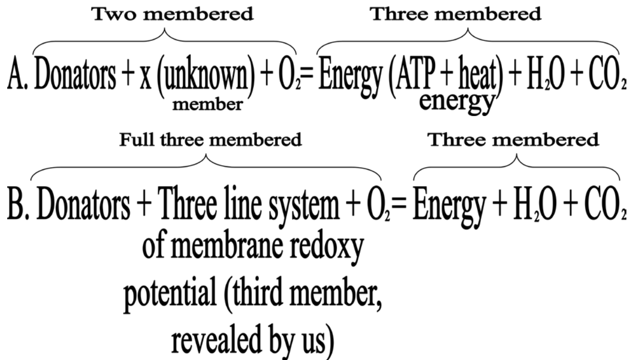
Figure 1. The membrane -redoxy potential three state line system between donators and acceptors inside the living cells.
